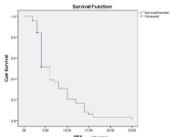
Fig. 2: PFS curve
